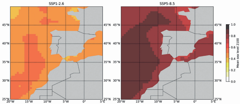
Figure 6.2. Median regional sea level change at 2100 for different scenarios (with respect to 1995–2014) for: (Left) SSP1-2.6; (Right) SSP5-8.5. These changes include all mechanisms that could be assessed with, at least, medium confidence (Intergovernmental Panel On Climate Change (ipcc), 2023) thereby excluding ice sheet processes associated with deep uncertainty.
