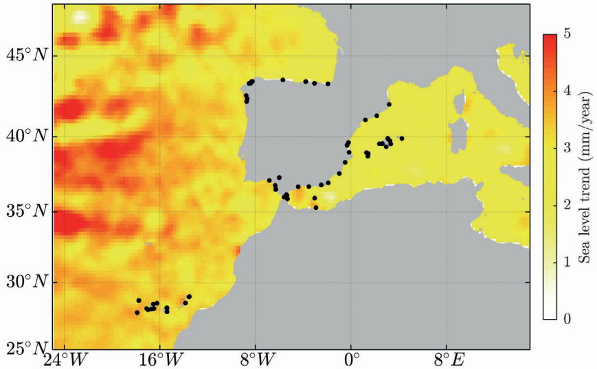
Figure 4.4. Absolute sea level trends from altimetry observations (1993-2023) and location of tide gauge stations along the Spanish coasts.
