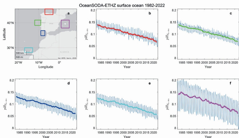
Figure 4.8. Temporal evolution of surface pH for the period 1982-2022 at different zones around Iberian Peninsula and Canary Islands. The zones are represented as squares in subplot (a) and the color code is shared with the time-series subplots (b-f). Data from OceanSODA-ETHZ (Gregor & Gruber, 2021).
