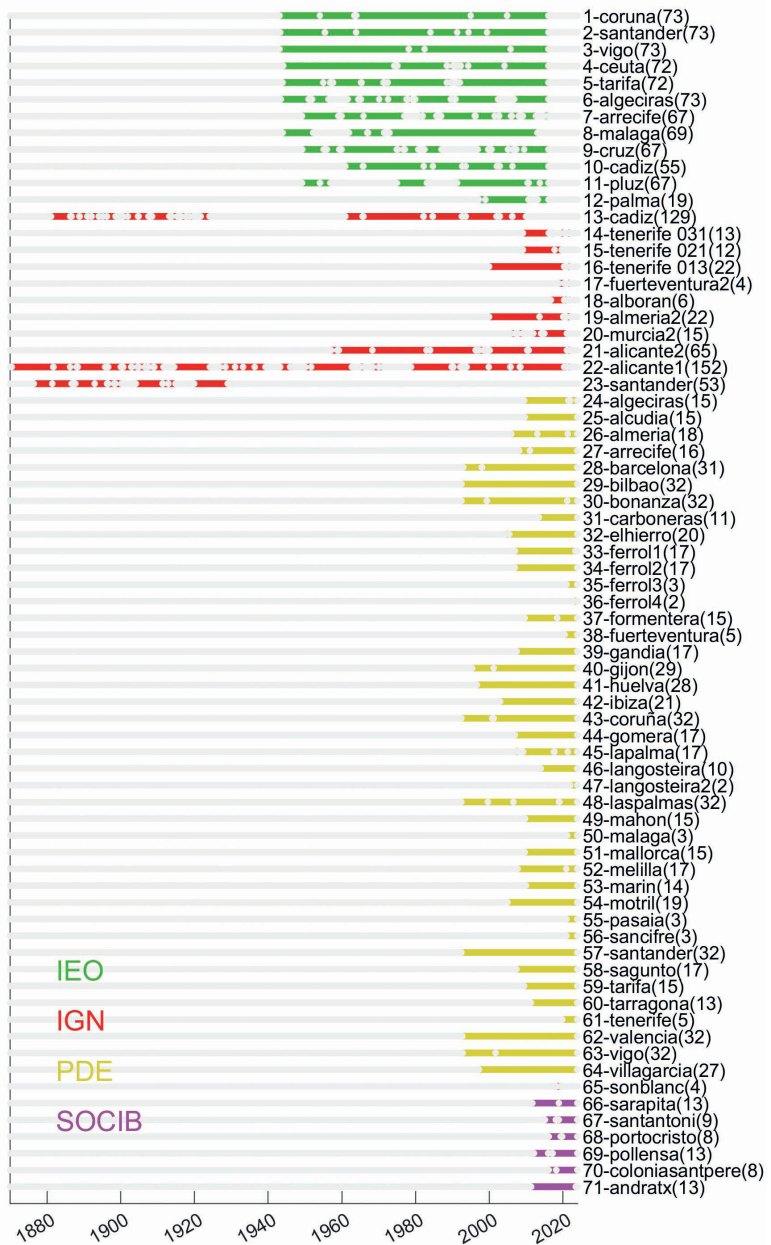
Figure 4.6. Spatio-temporal distribution of tide gauge observations along the Spanish coasts.
