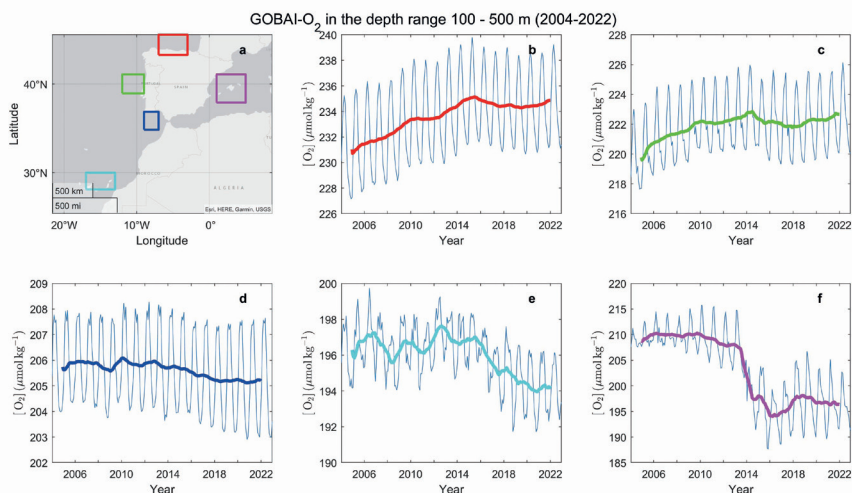
Figure 4.9. Mean concentration of dissolved oxygen [ O_2 ] ( \mu\text{mol kg}^{-1} ) in the depth layer 100-500 m for the period 2004-2022 at different zones around Iberian Peninsula and Canary Islands. The zones are represented as squares in subplot (a) and the color code is shared with time-series subplot (b-f). Note that the y-axis is not the same for each subplot. Data from GOBAI-O 2 (Sharp et al., 2023).
