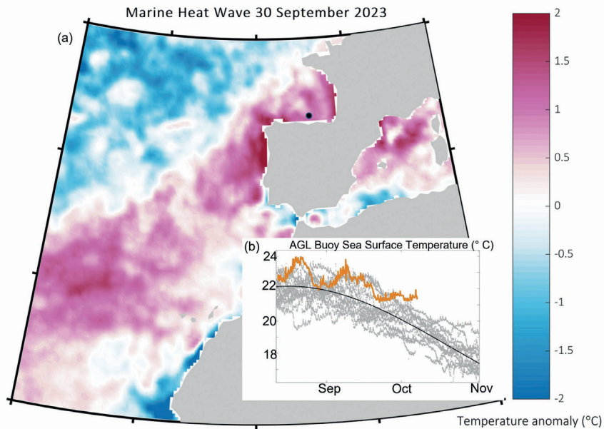
Figure 4.3. (a) Marine heat wave in the eastern North Atlantic and Western Mediterranean detected from satellite-derived sea surface temperature data (NOAA OI SST V2 High Resolution Dataset, https://psl.noaa.gov/data/gridded/data.noaa.oisst.v2.highres.html ) following Hobday et al., 2016 at the end of September 2023, where after the summer temperatures were between 1.5 and 2°C above the 90th percentile of sea surface temperature. The black dot in (a) marks the location of the AGL buoy in the Bay of Biscay. (b) Sea surface temperature recorded by the buoy from mid-August to mid-October (orange line) in comparison with remaining data recorded by AGL buoy for the same days of the year since its deployment in 2007 (gray dots) and its annual climatological cycle (black line).
