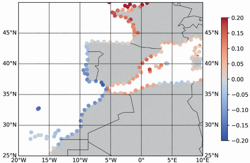
Figure 6.4. Impact of storm surges and waves on changes (increase/decrease) in the 95 th percentile of ESL (m) by 2100, relative to baseline period (1980–2014) for the European coastline (adapted from Jevrejeva et al., 2023). This contribution should be added to the mean sea-level rise to obtain the total change of ESL.
