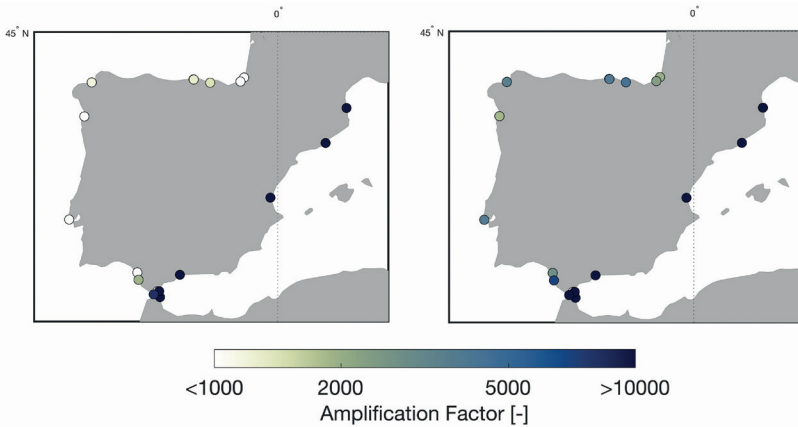
Figure 6.3. Projected median frequency amplification factors of the historical centennial sea level event in 2100 under the SSP2-4.5 and SSP5-8.5 scenario (adapted from Intergovernmental Panel On Climate Change (IPCC, 2023)). An amplification factor of 100 means that events occurring every 100 years on average, could occur every year.
