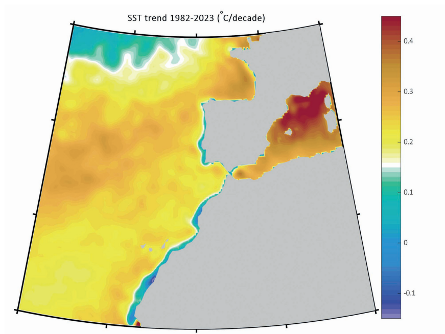
Figure 4.1. SST trends from NOAA OI SST V2 High Resolution Dataset ( https://psl.noaa.gov/data/gridded/data.noaa.oisst.v2.highres.html ) or the satellite-derived SST period 1982-2023. SST trends are indicated by the color scale. White color marks the averaged global SST warming trend ( 0.15\text{ }^{\circ}\text{C/decade} ) for the period 1980-2020 as reference. As observed, with the only exception of some coastal waters, all oceanic waters surrounding the Iberian Peninsula and archipelagos are warming faster than the global average.
