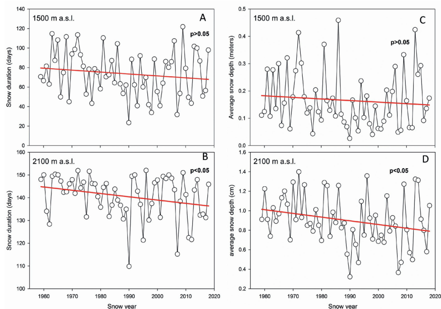
Figure 2.4: Evolution of annual snow cover duration (a, b) and average snow depth from December to April (c, d) at 1,500 and 2,100 m., respectively (López-Moreno et al., 2020a).
