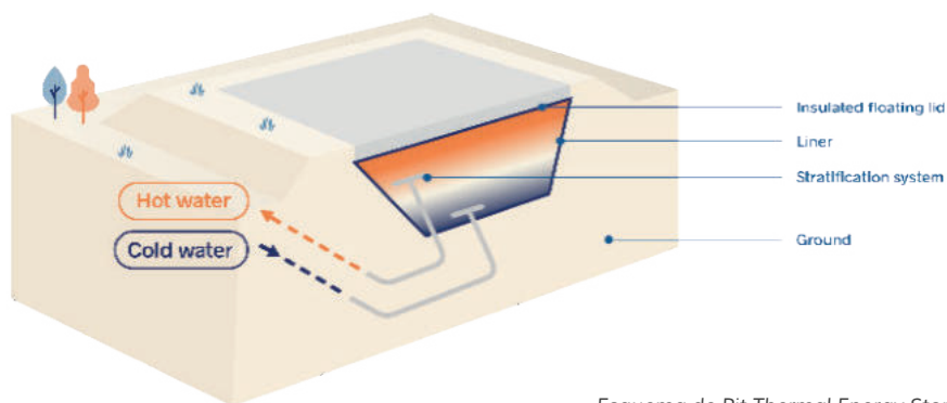
Esquema de Pit Thermal Energy Storage (PITES) (© Newheat)
